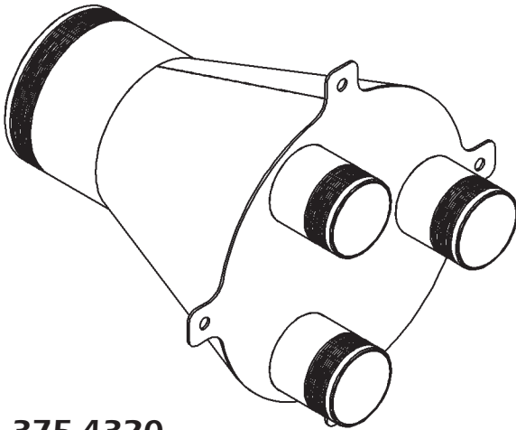
375-4320 4" Inlet x 3 - 2" Outlets
