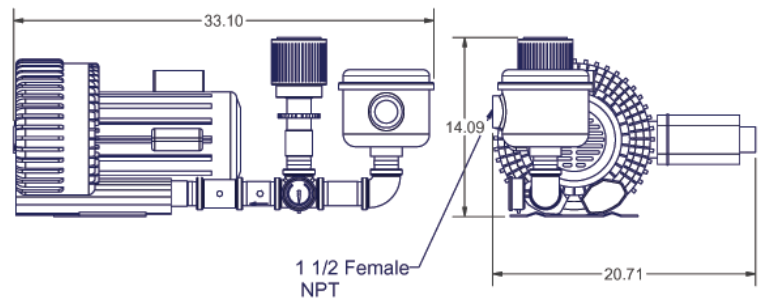
Kit Vacuum Pump 1 1/2" NPT KVHRB402-1
