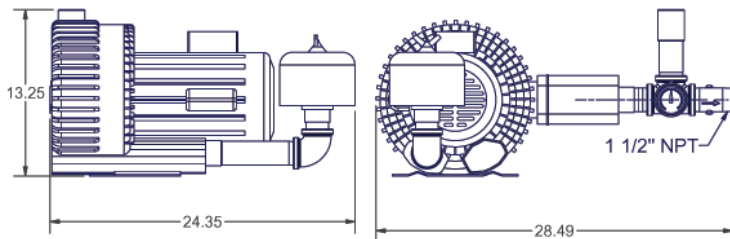
Kit Pressure Pump 1 1/2" NPT KPHRB402-1
