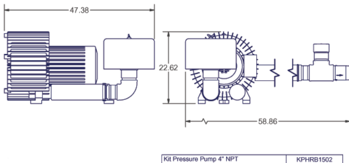
KPHRB1502 - Pressure Kit Drawing
