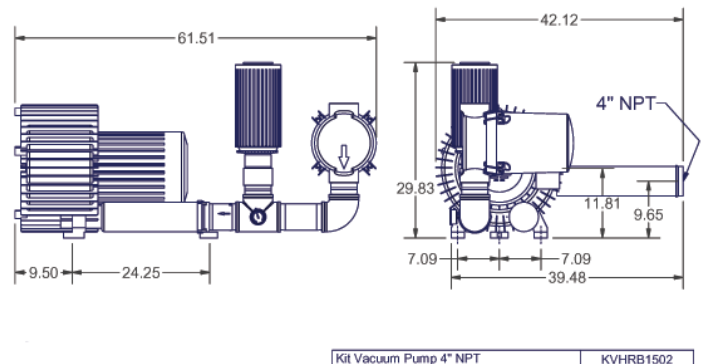
KVHRB1502 - Vacuum Kit Drawing
