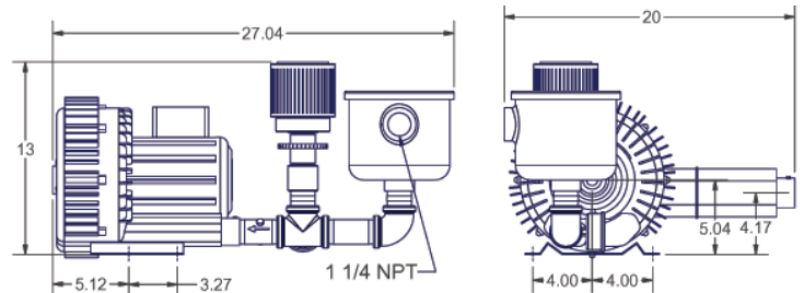
Kit Vacuum Pump 1 1/4" Kit KVHRB102
