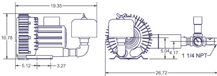
Kit Pressure Pump 1 1/4" NPT KPHRB102
