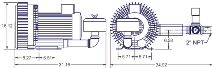
Kit Pressure 2" NPT KPHRB1002
