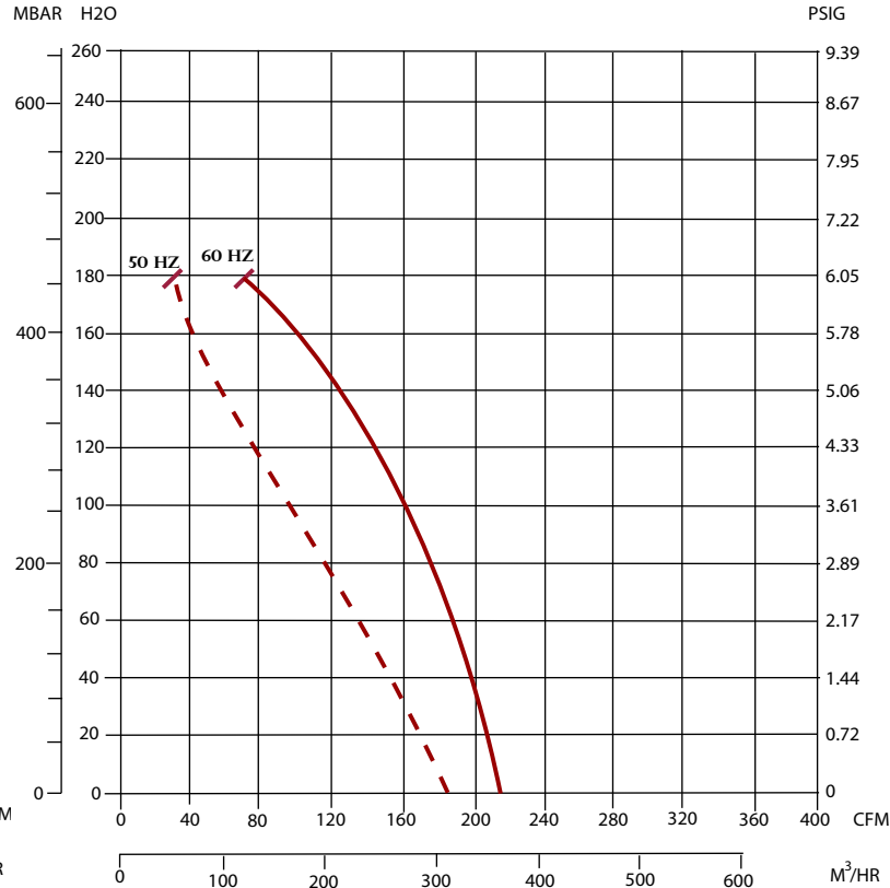
Vacuum vs. CFM
