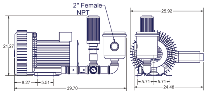
KVHRB1002 - Vacuum Kit Drawing
