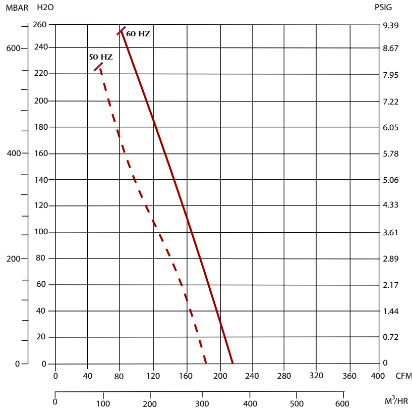
Pressure vs. CFM
