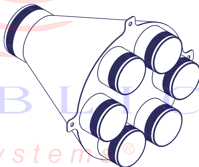
375-4630 4" Inlet x 6 - 3" Outlets
